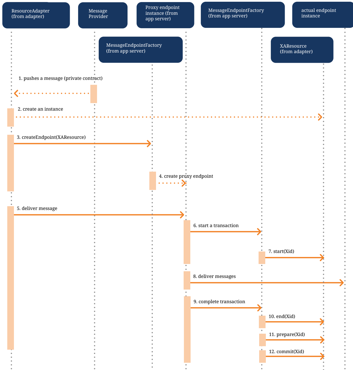
Transacted Message Delivery: Option B (Sequence Diagram)
